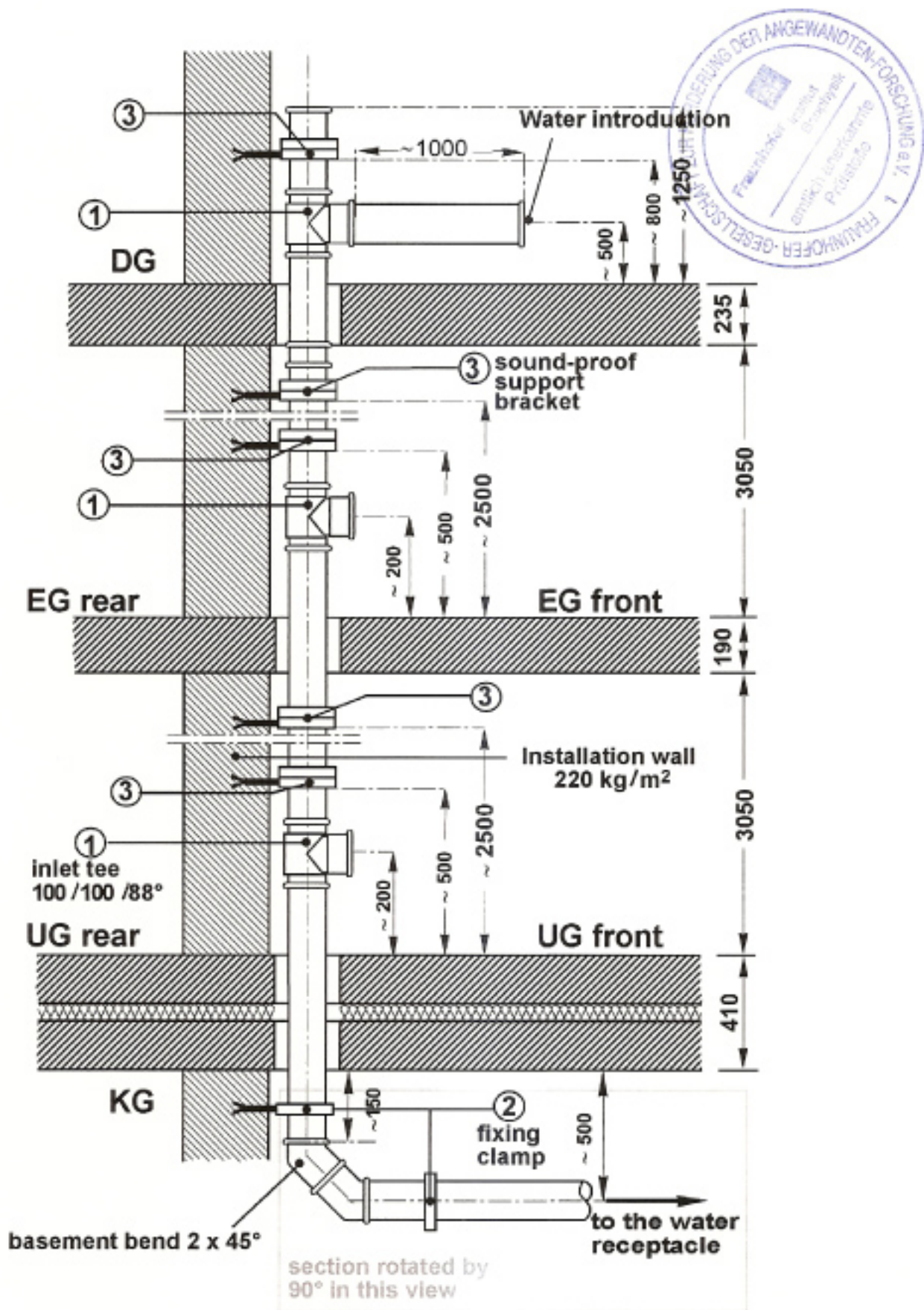
Figure 4 Installation plan of the pipe system "TERRAIN SDP INSONORIZADO PVC, 110x5.3", mounted with clamps "sound proof support bracket" manufactured by REHAU (drawing not to scale, dimensions in mm).
