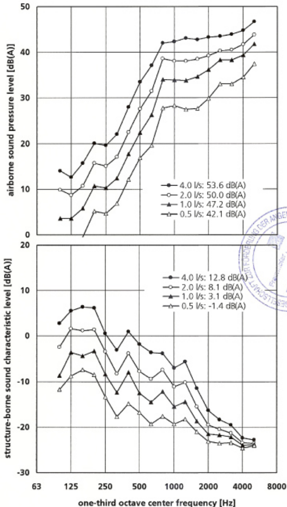
Figure 2 Wastewater pipe system *TERRAIN SDP INSONORIZADO PVC, 110x5.3" mounted in sub-basement (KG), basement (UG front), ground floor (EG front) and top floor (DG) using pipe clamps *sound proof support bracket" (manufacturer: REHAU). Airborne sound pressure level (above) and structure-borne sound characteristic level (below) measured at various flow rates according to EN 14366.
