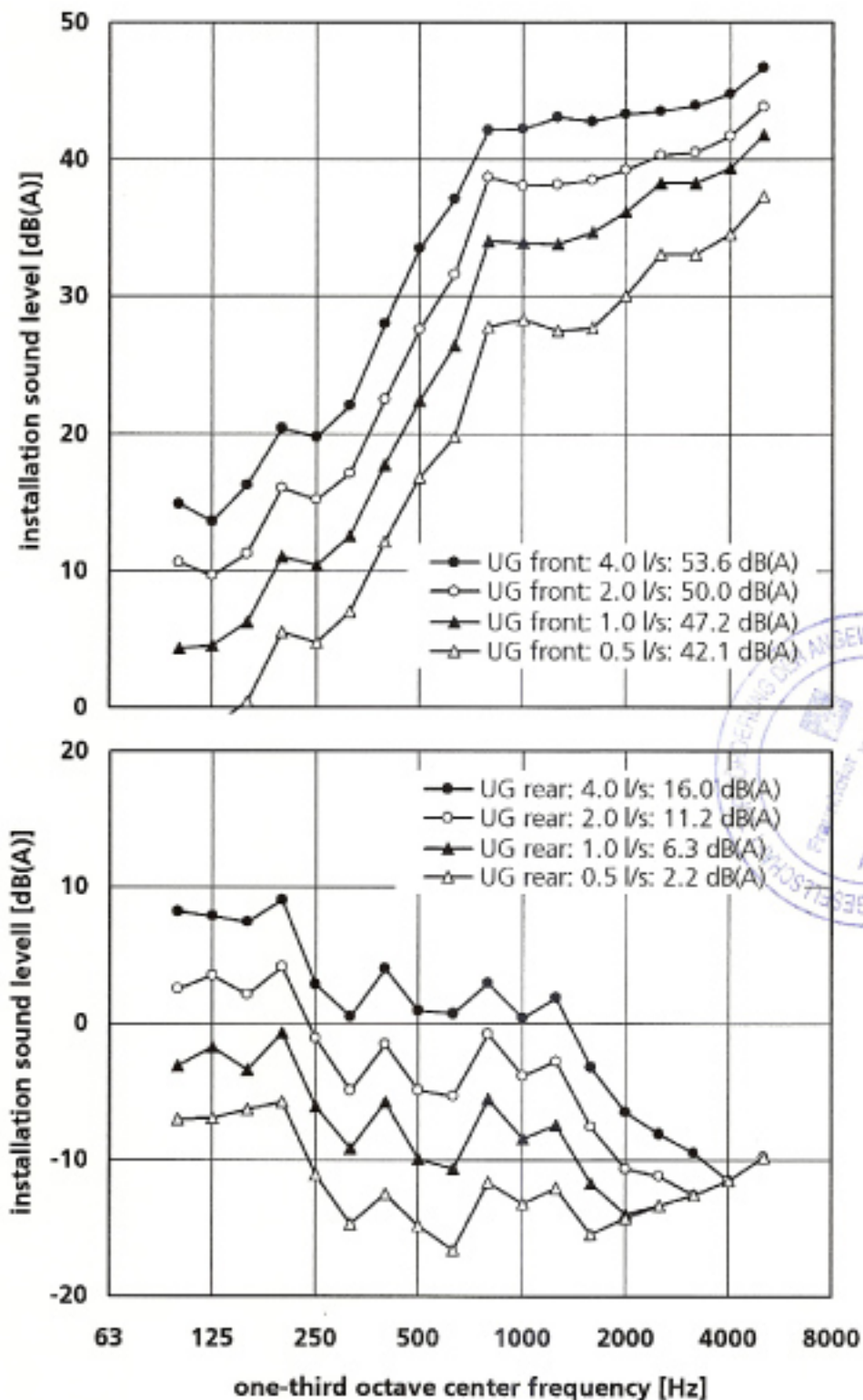
Figure 1 Wastewater pipe system "TERRAIN SDP INSONORIZADO PVC, 110x5.3" mounted in sub-basement (KG), basement (UG front), ground floor (EG front) and top floor (DG) using pipe clamps "sound proof support bracket" (manufacturer: REHAU). The installation sound level L_{in} was measured at various flow rates in the test rooms UG front (above) and UG rear (below).
